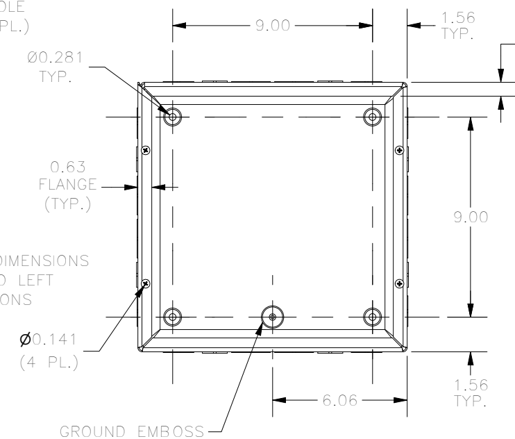
FRONT VIEW LID REMOVED
