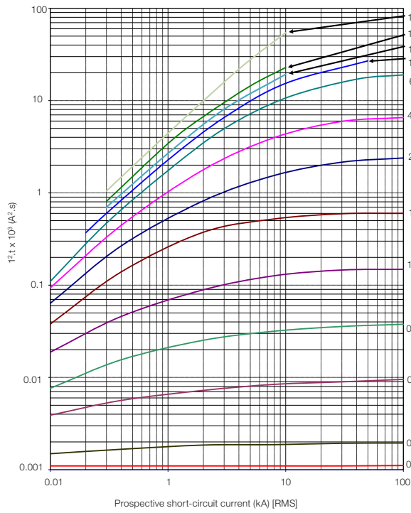
I 2 t at 415 V - MPW12/18 and MPW18i
