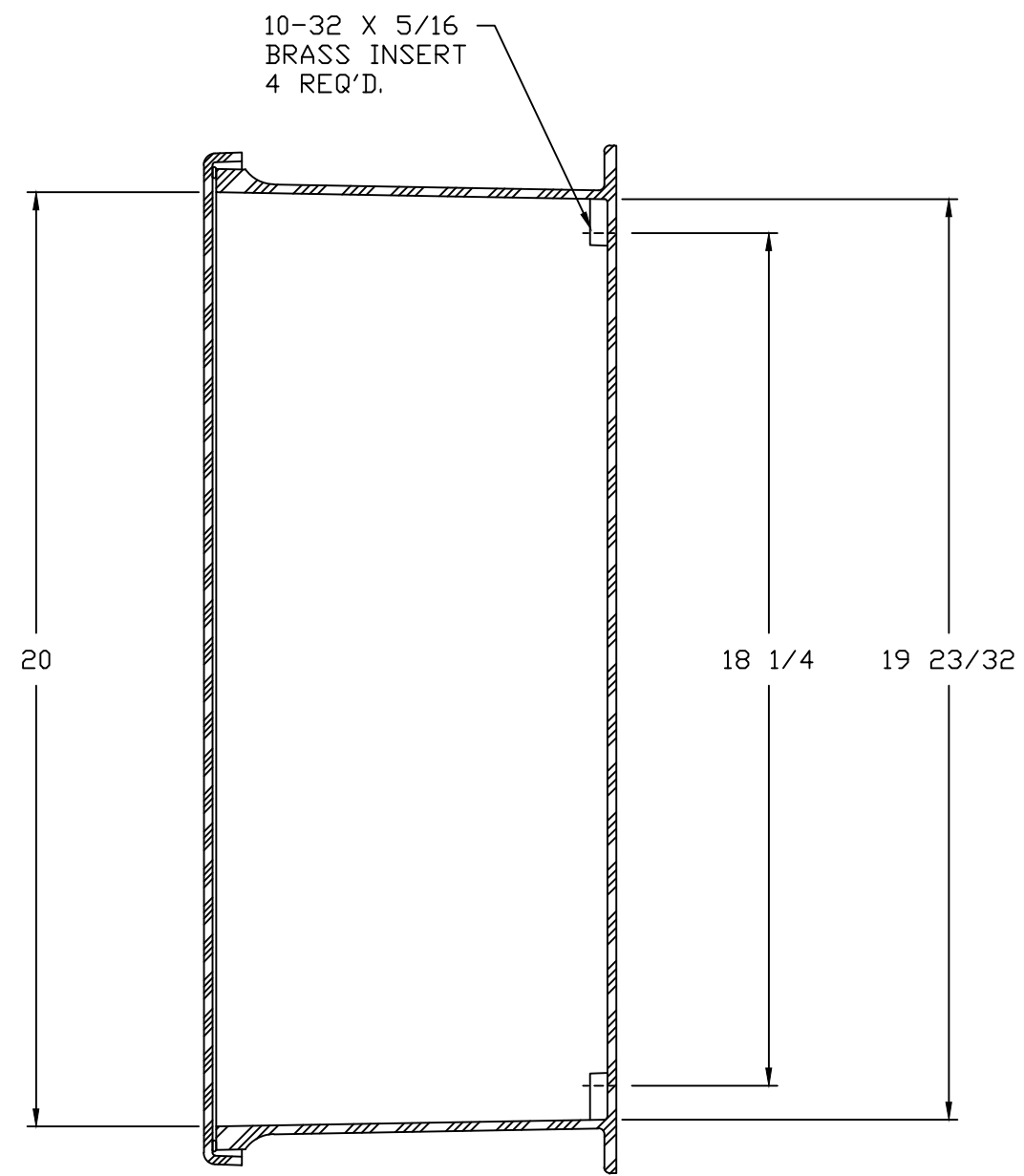
SECTION B-B
