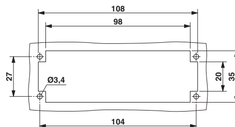
Mounting cutout
