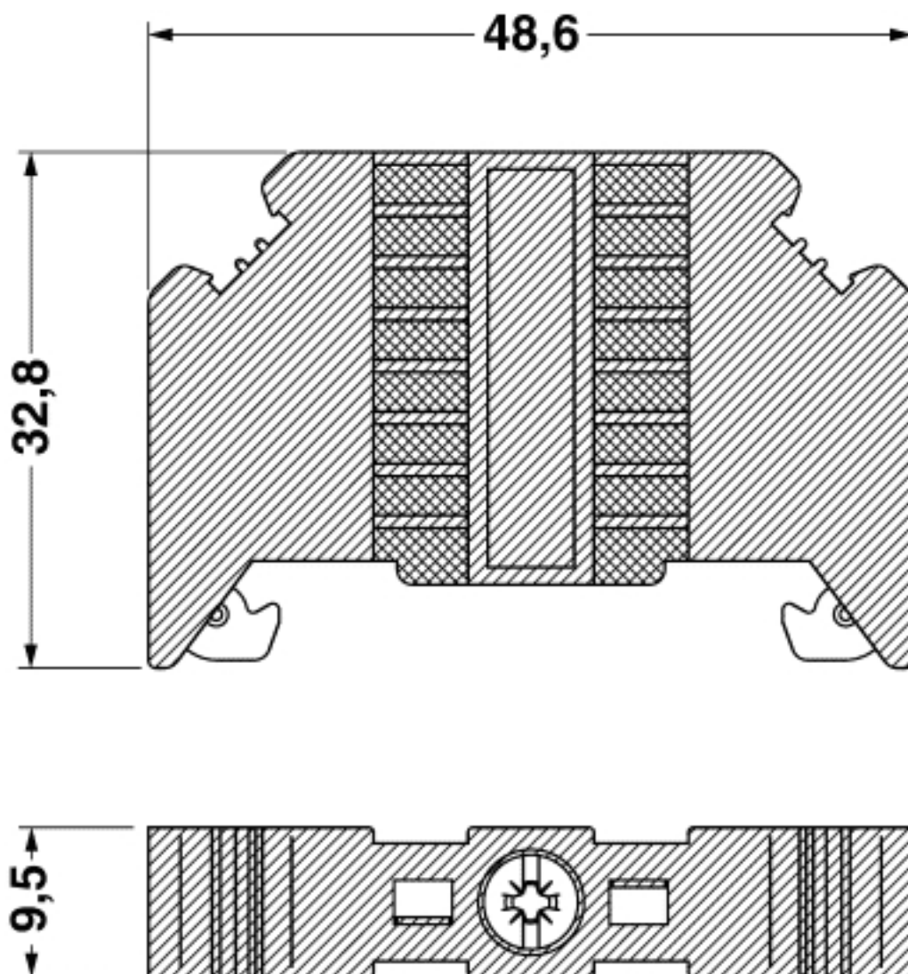
Dimensional drawing
