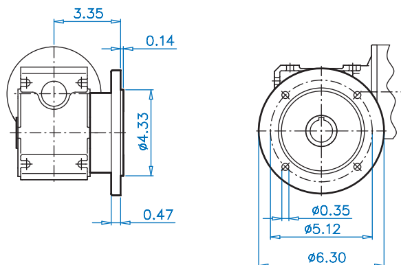
SK 1SI50 F (III Flange)
