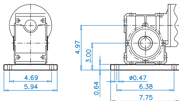
SK 1SI50 H (Shaft Cover)
