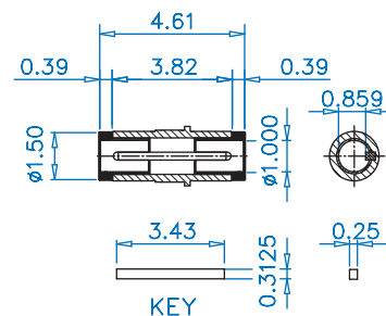
SK 1SI50 J (1.00" Bushing Kit)
