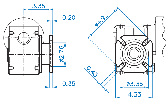
SK 1SI50 F (II Flange)
