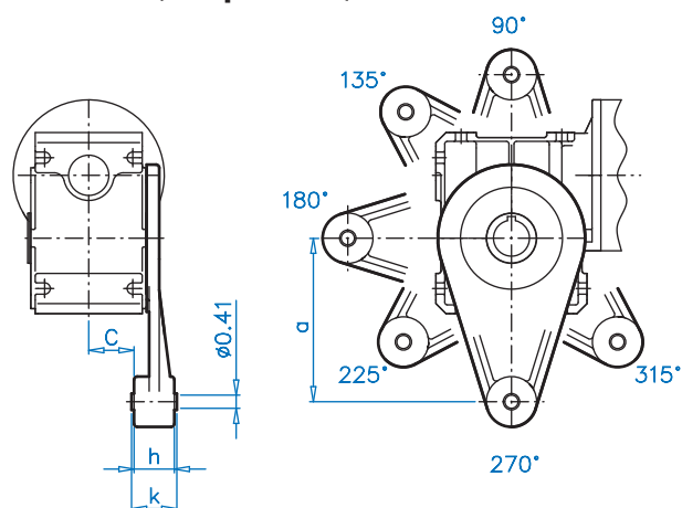
SK 1SI50 D (Torque Arm)
