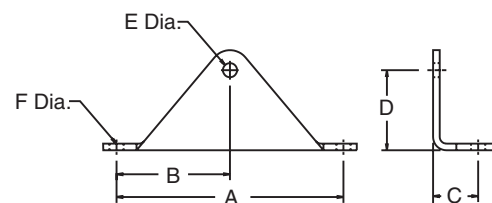
375-600 Torque Arm Kit
