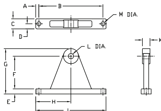
133-325 Torque Arm Kit
