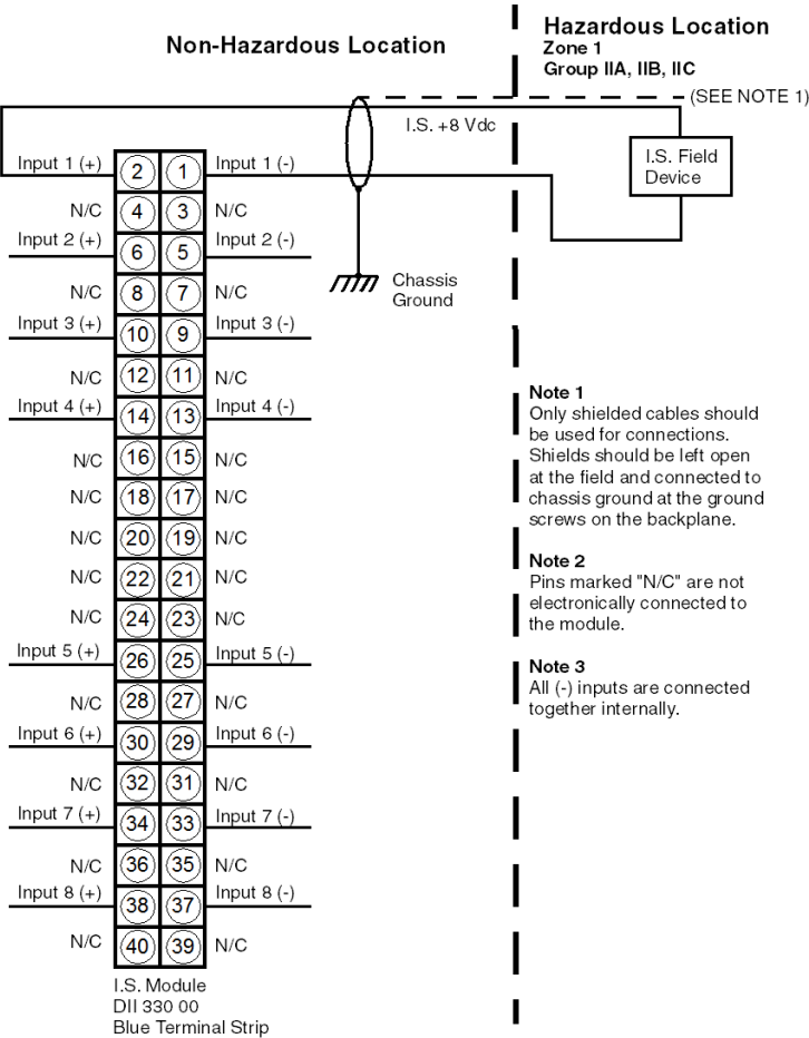
140 DII 330 00 Wiring Diagram
