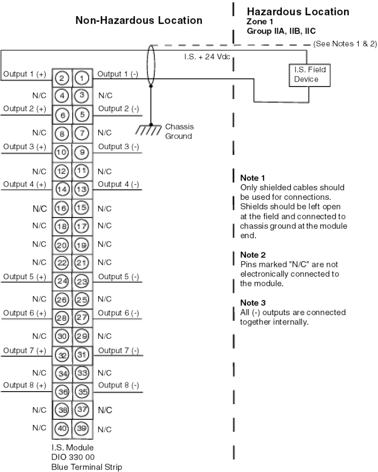
140 DIO 330 00 Wiring Diagram
