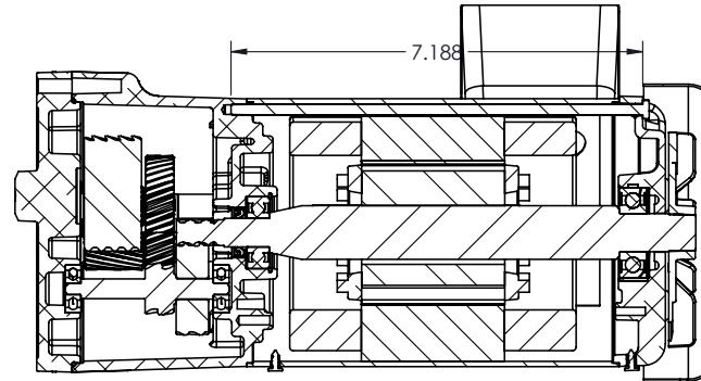
SECTION R-R
