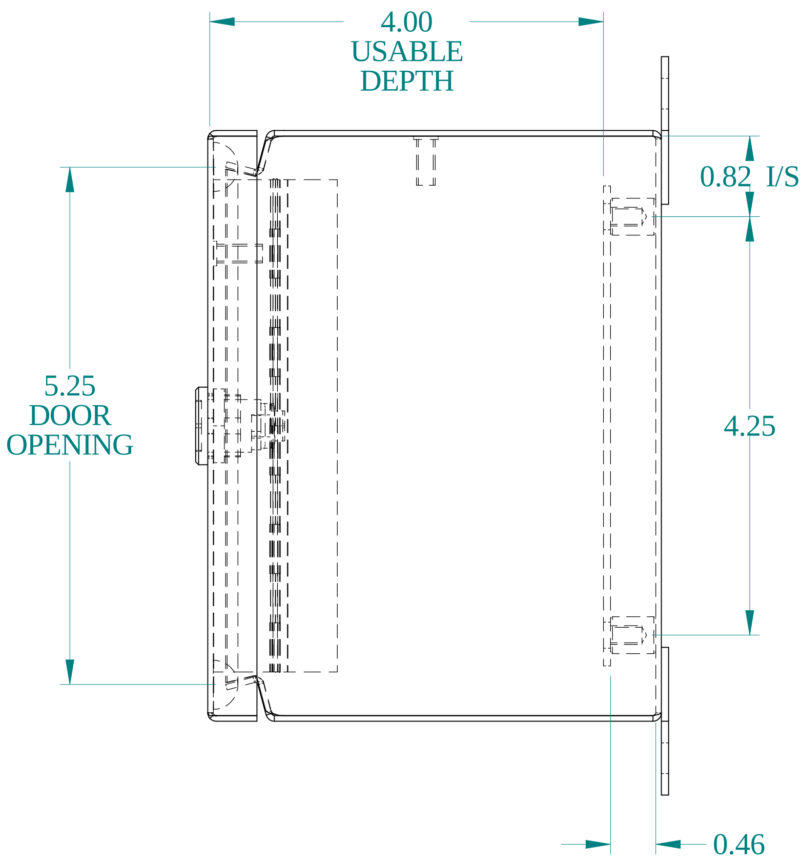
SIDE VIEW
