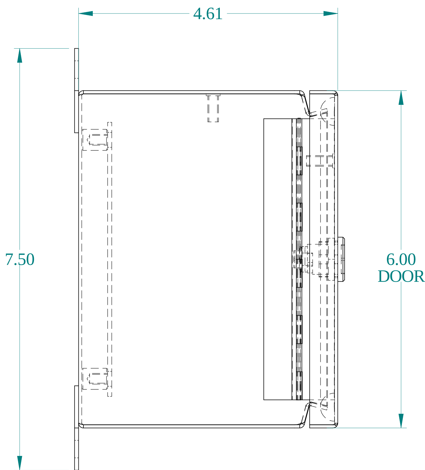
SIDE VIEW
