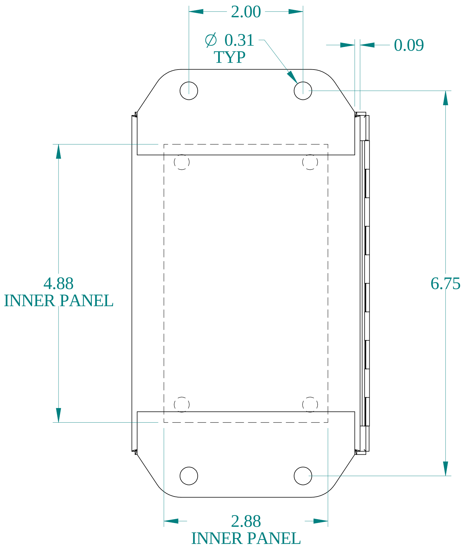
BACK VIEW
