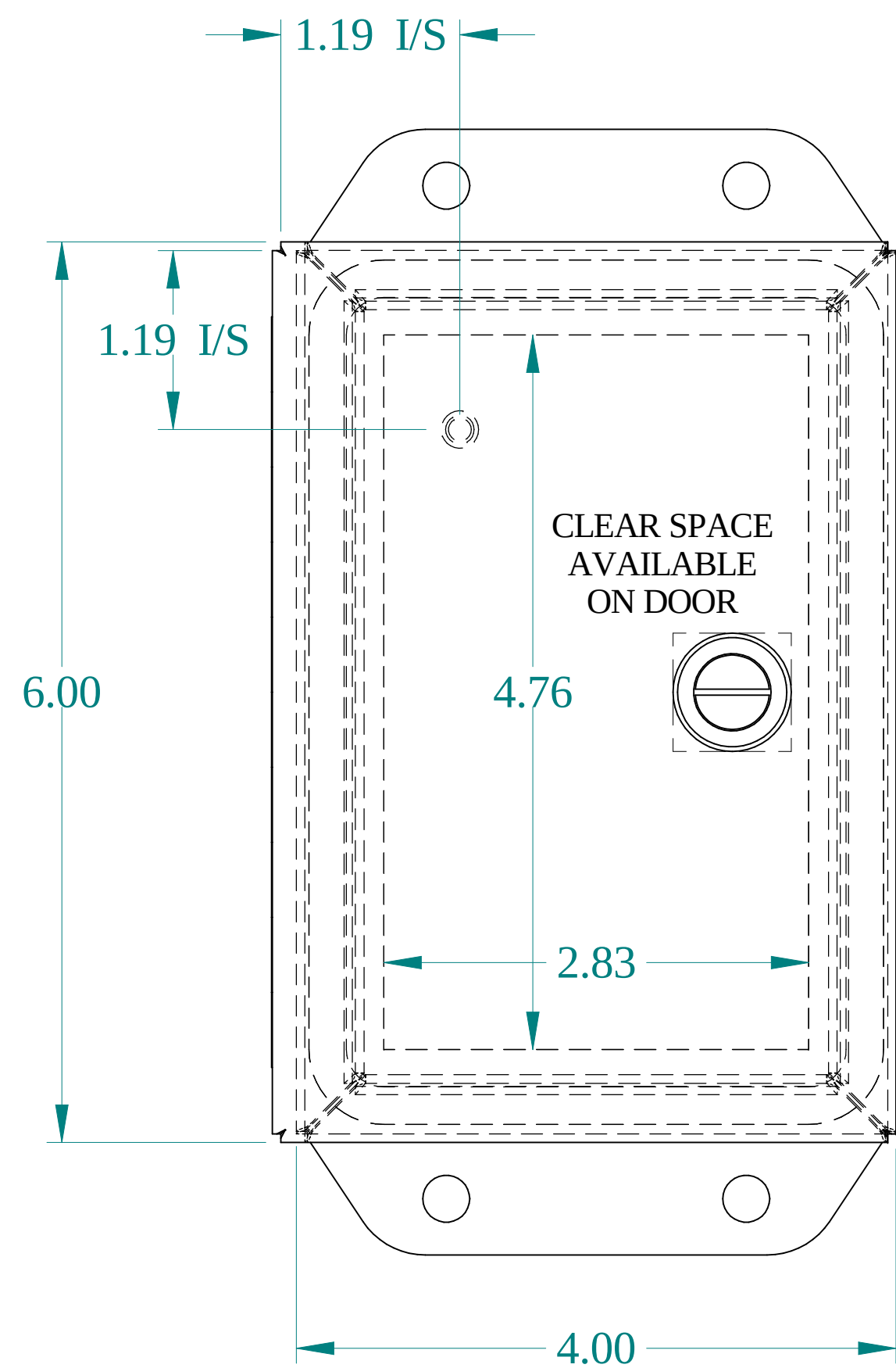
FRONT VIEW
