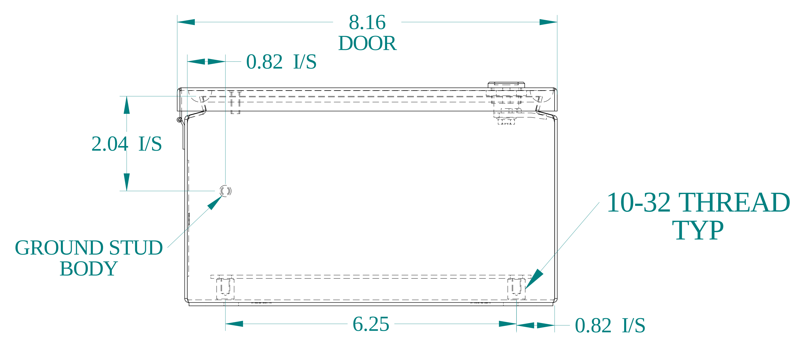
BOTTOM VIEW
