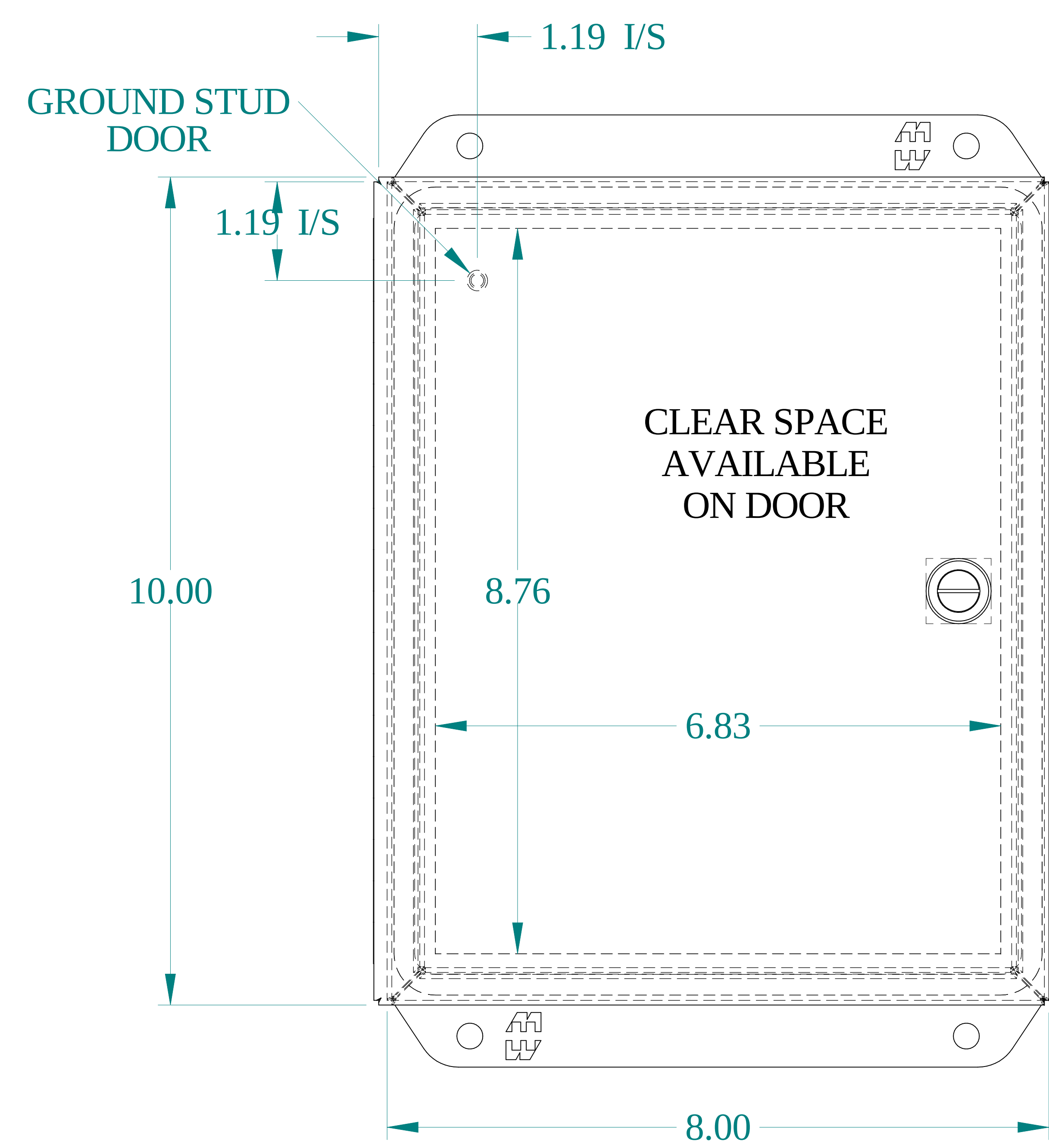
FRONT VIEW
