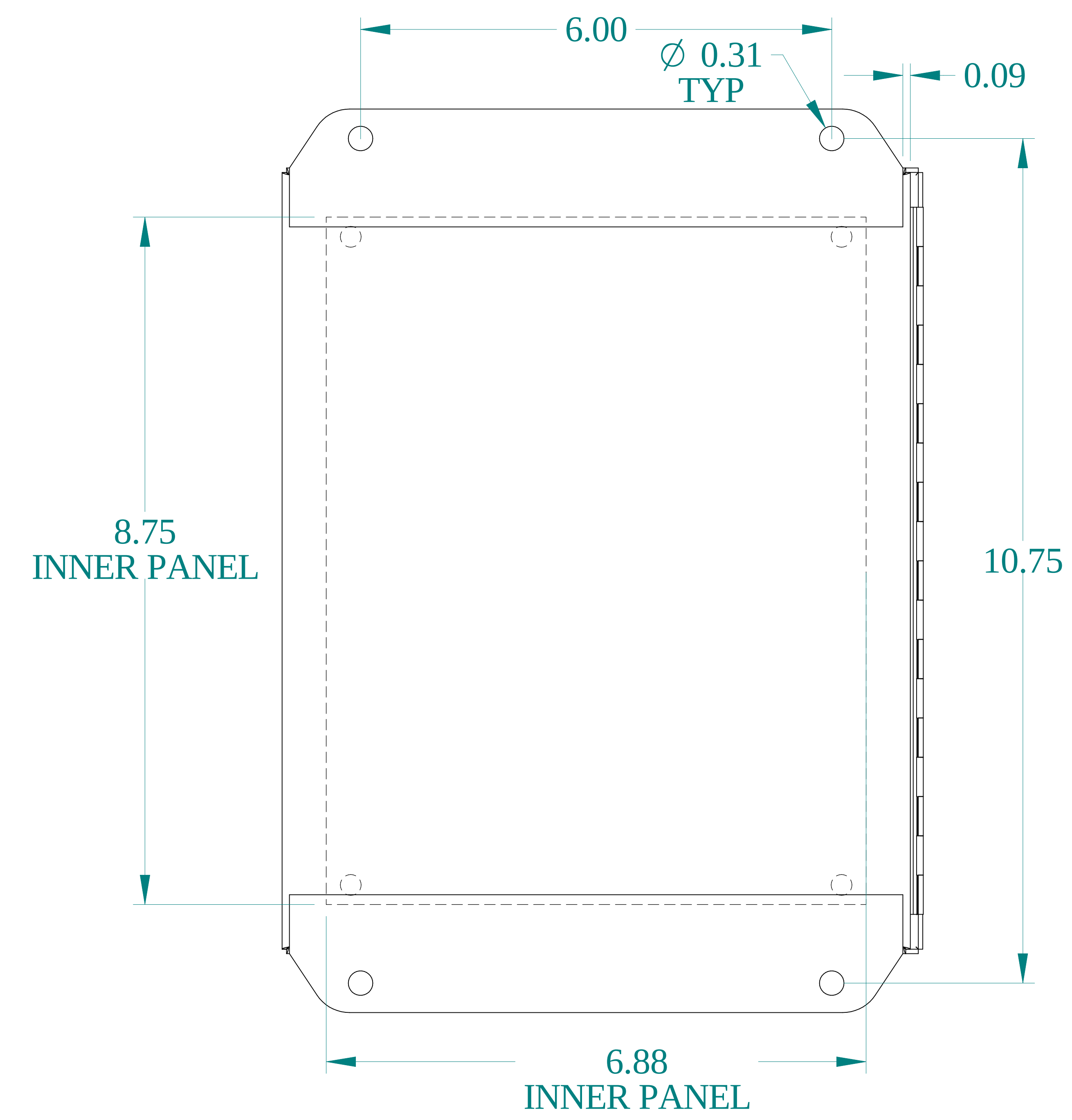
BACK VIEW
