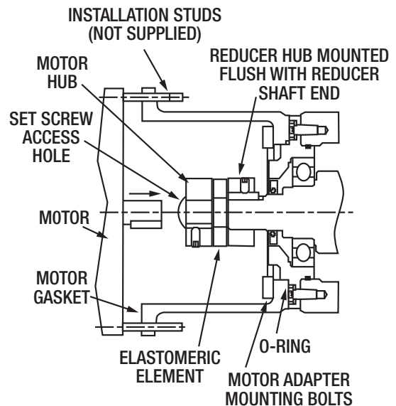
Figure 2 - Motor Mounting
