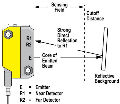
Figure 8. Reflective Background - Problem
