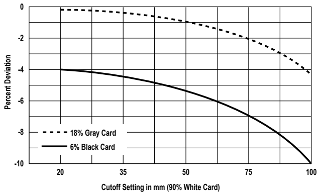
Figure 3. QS18AF cutoff point deviation
