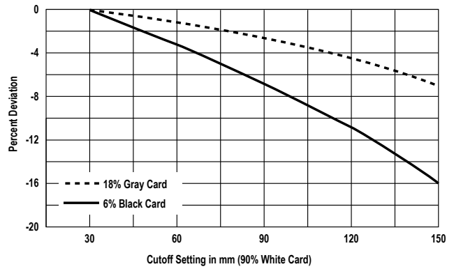
Figure 4. QS18LAF cutoff point deviation
