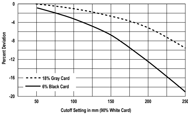
Figure 5. QS18LAF250 cutoff point deviation
