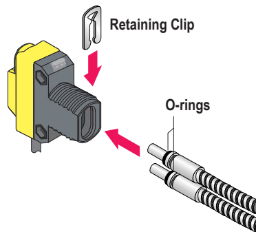
Figure 3. Installing Glass Fibers
