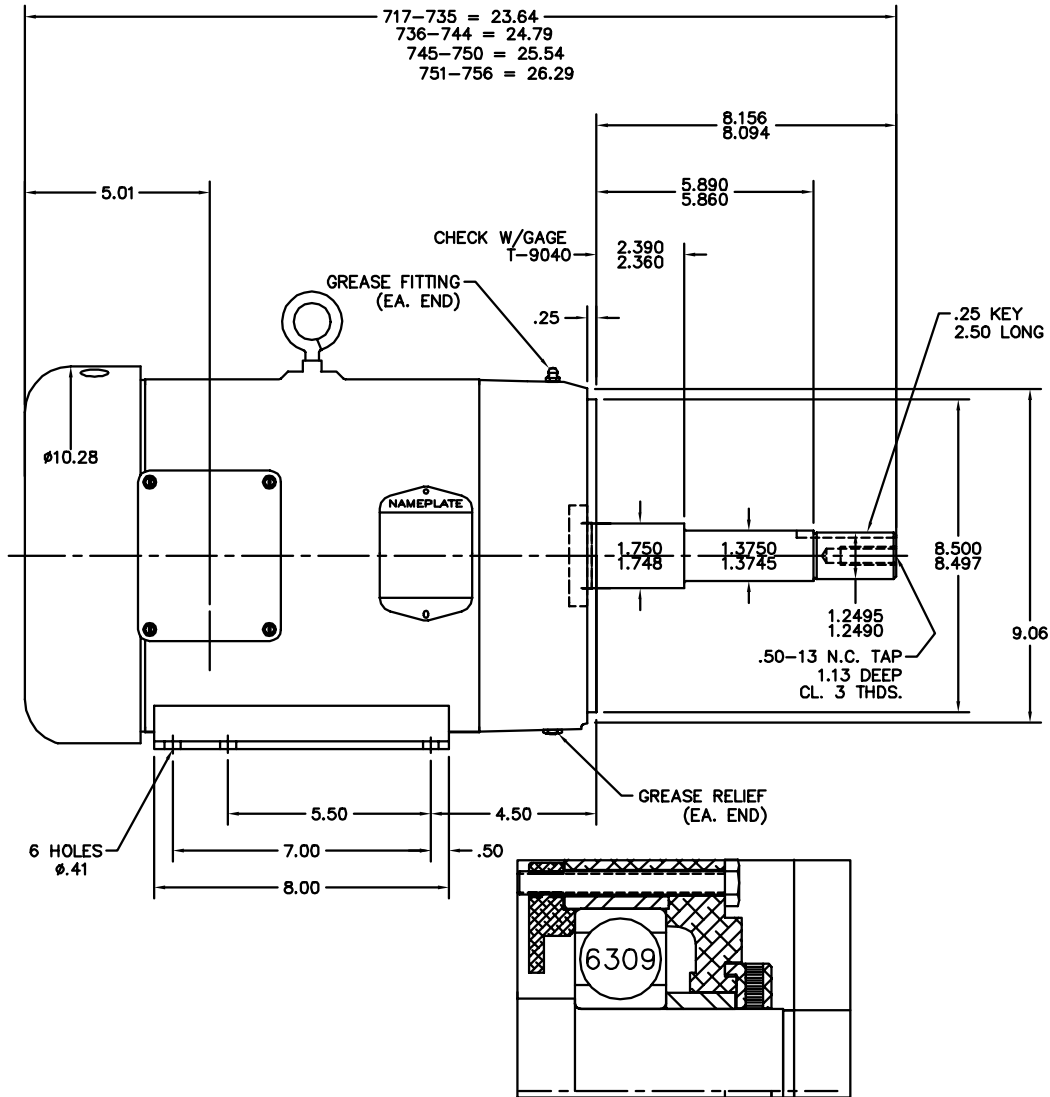
PULLEY END DETAIL
