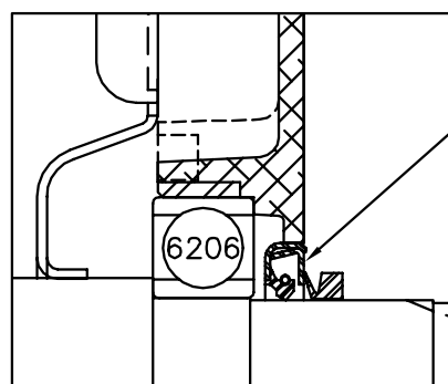
PULLEY END DETAIL
