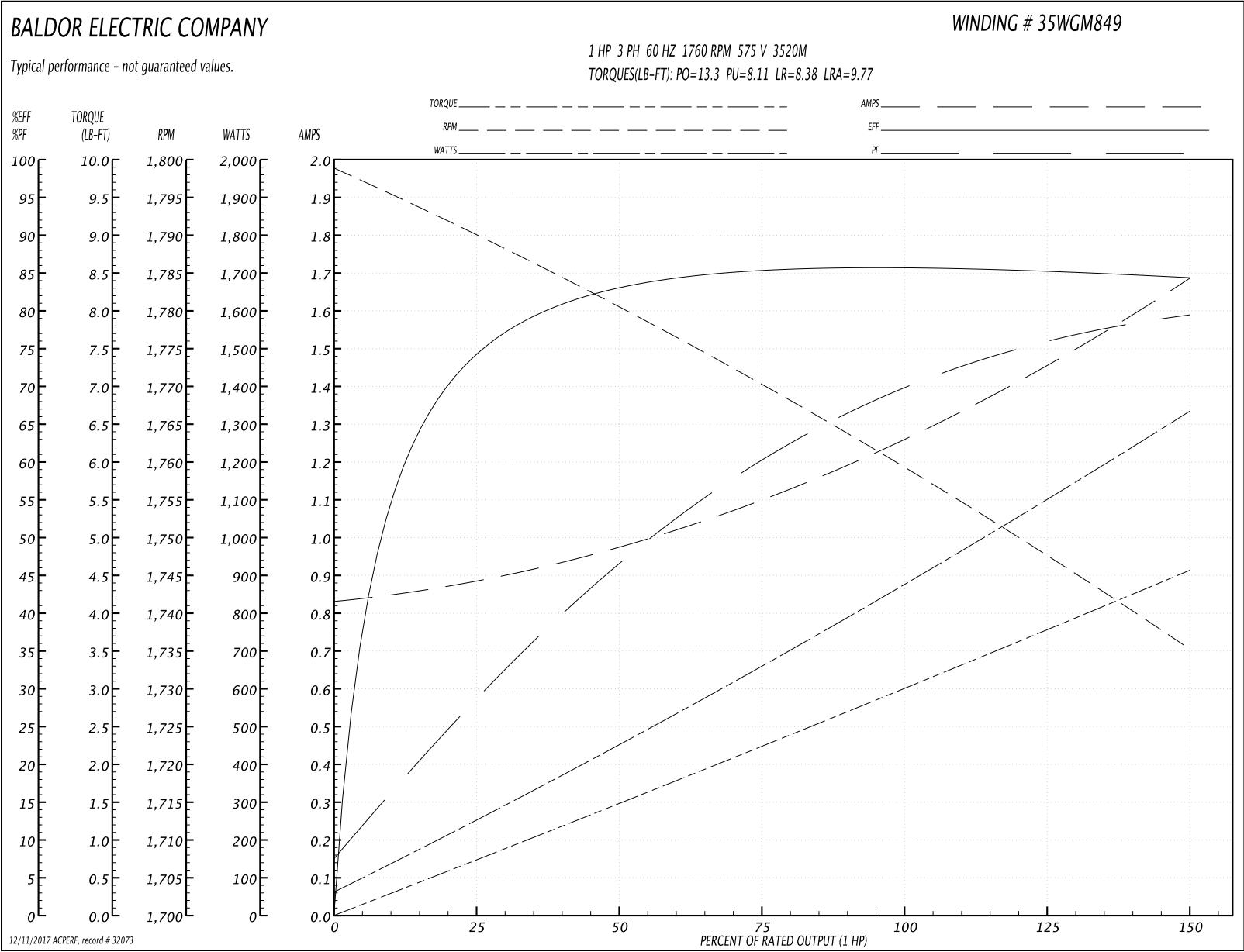
Performance Graph at 575V, 60Hz, 1.0HP Typical performance - Not guaranteed values
