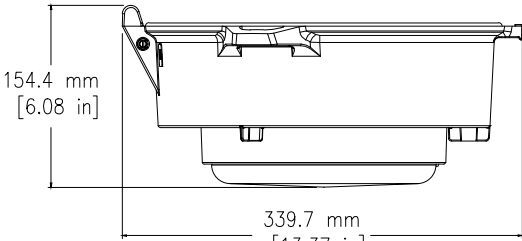
Side View - Globe
