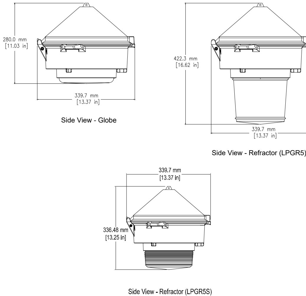
FIGURE 7: LUMINAIRE WITH PENDANT CONE
