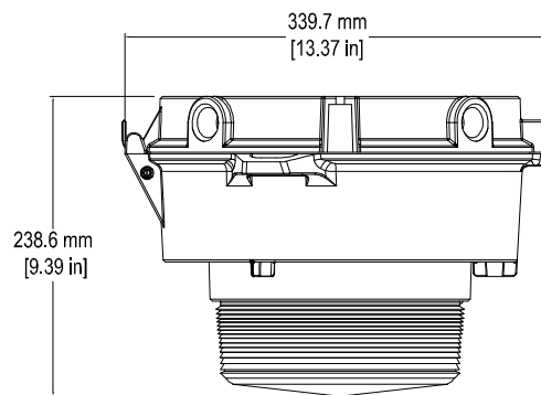
Side View - Refractor (LPGR5S)
