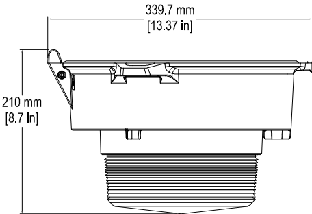
Side View - Refractor (LPGR5S)
