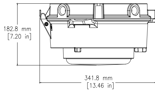
Side View - Globe
