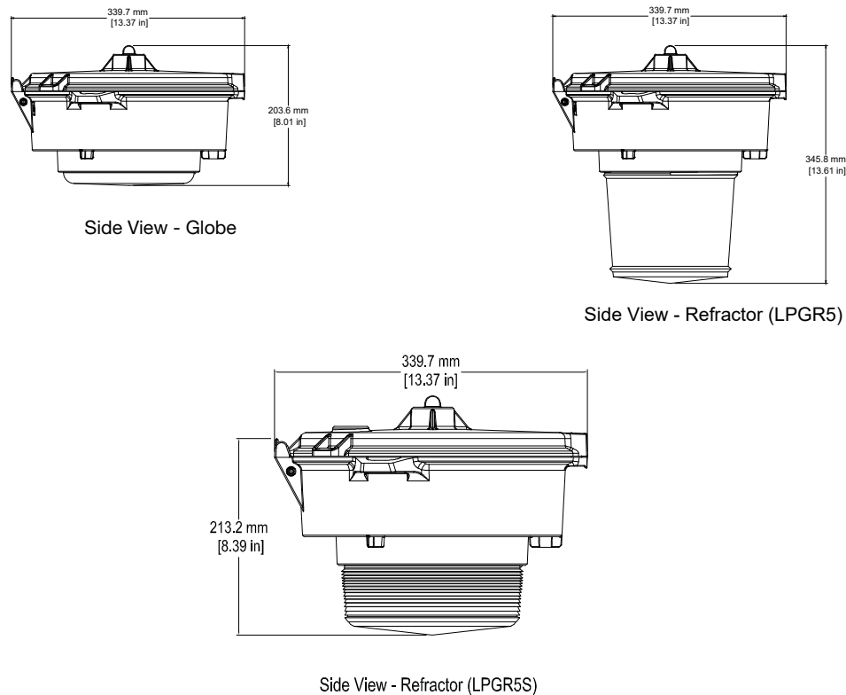
FIGURE 4: LUMINAIRE WITH WATERTIGHT PENDANT HOOD
