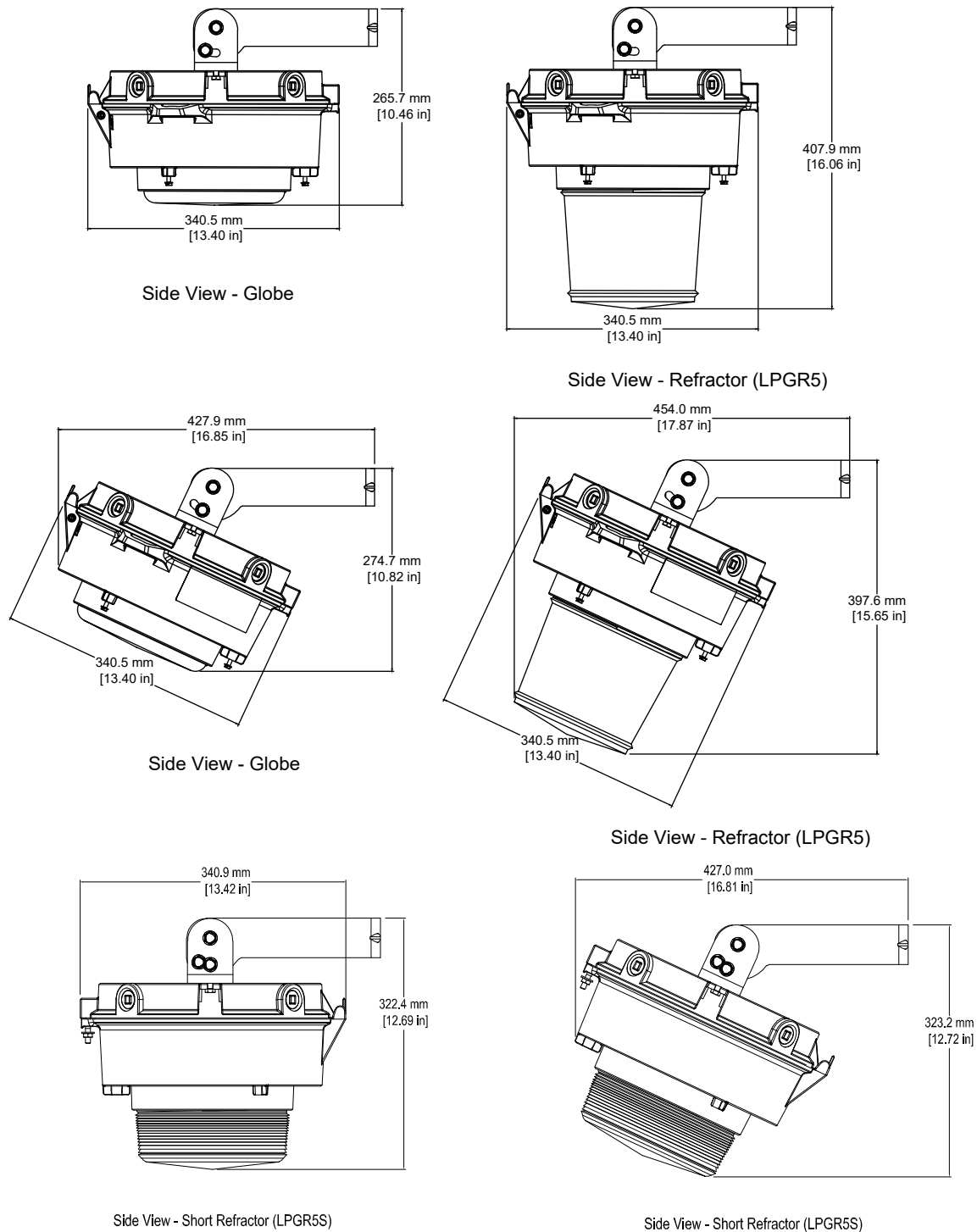
FIGURE 11: LUMINAIRE WITH TRUNNION HOOD
