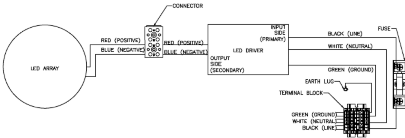
FIGURE 21: LUMINAIRE WITH OPTIONAL FUSE
