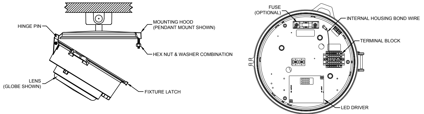
FIGURE 19: WIRING COMPARTMENT
