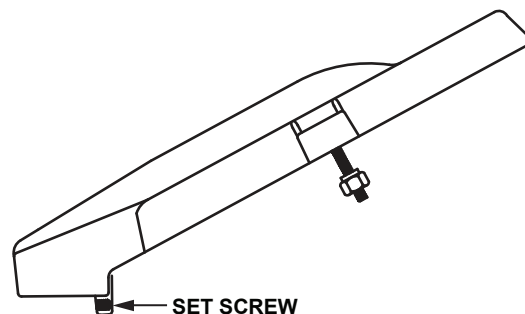
FIGURE 16: 25° STANCHION HOOD DETAILS
