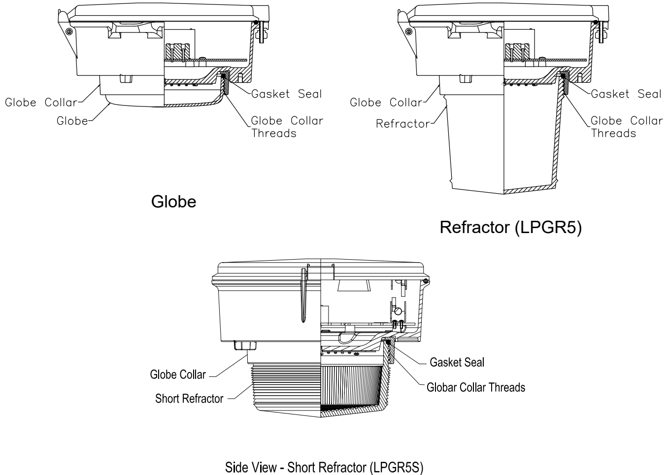
FIGURE 24: GLOBE/REFRACTOR SEALING DETAIL
