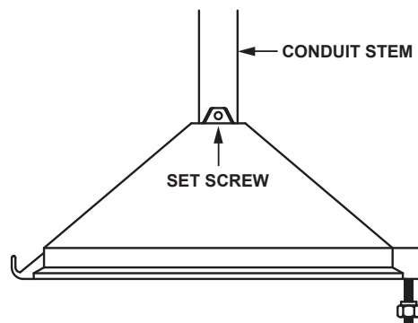
FIGURE 8: PENDANT CONE HOOD DETAILS
