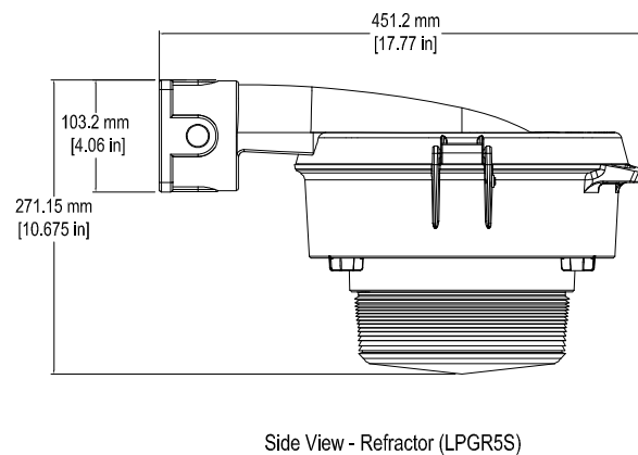
FIGURE 13: LUMINAIRE WITH WALL HOOD
