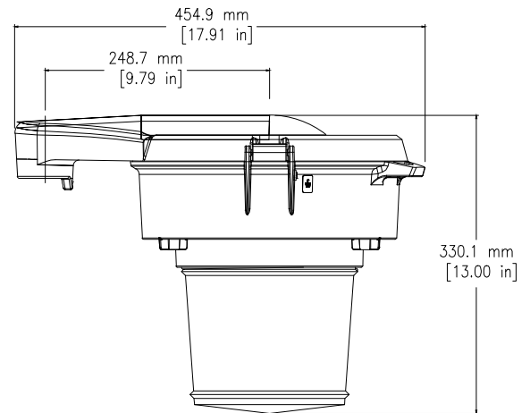
Side View - Refractor (LPGR5)
