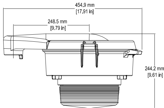
Side View - Refractor (LPGR5S)
