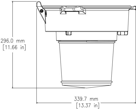
Side View - Refractor (LPGR5)
