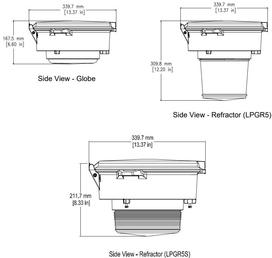
FIGURE 2: LUMINAIRE WITH PENDANT HOOD
