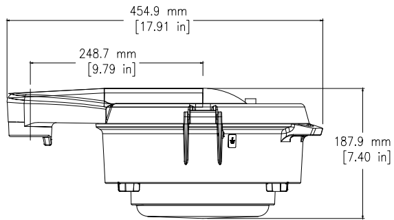
Side View - Globe
