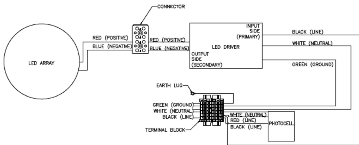
FIGURE 22: LUMINAIRE WITH OPTIONAL PHOTOCONTROL
