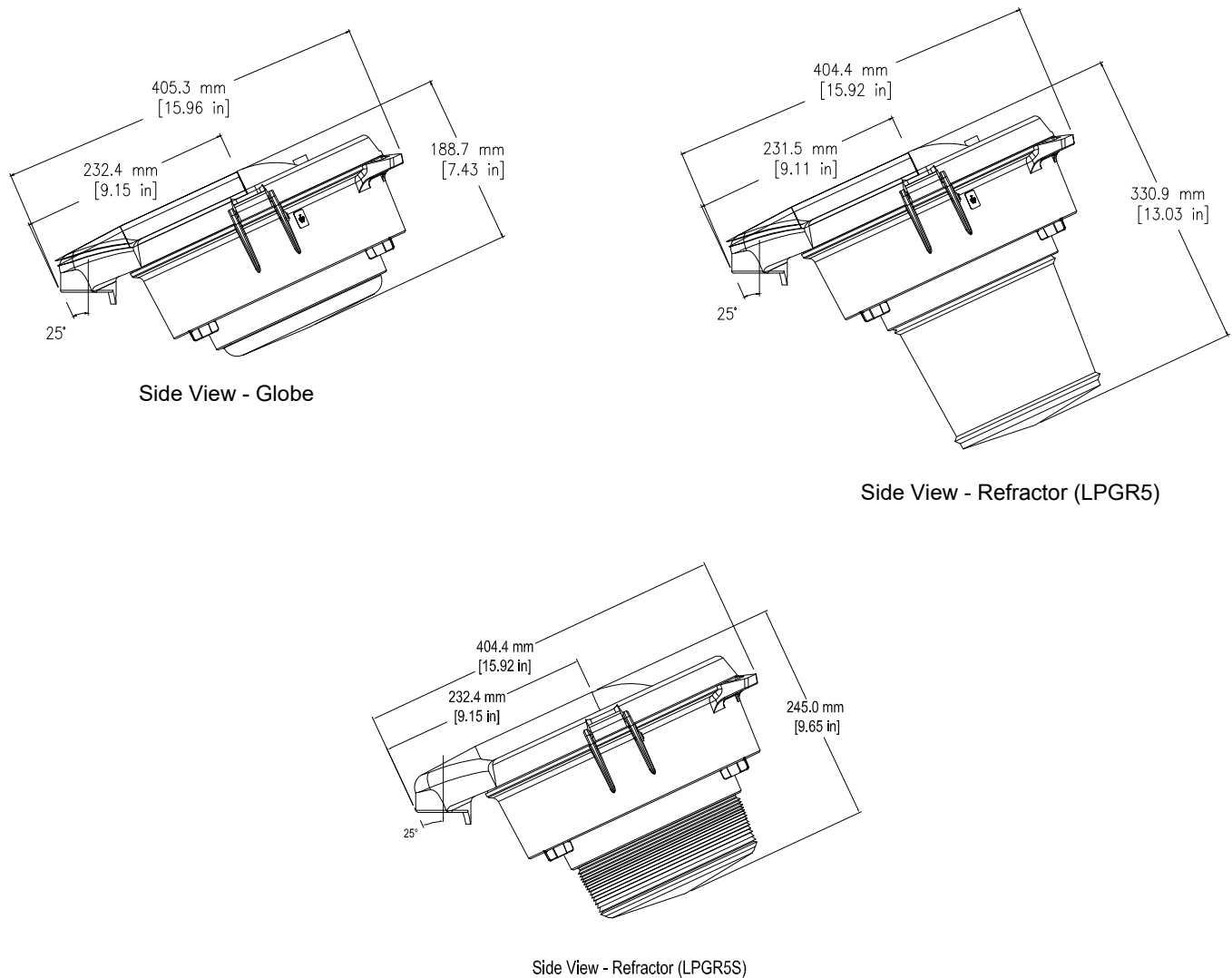
FIGURE 15: LUMINAIRE WITH 25° STANCHION HOOD
