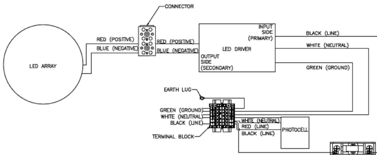
FIGURE 23: LUMINAIRE WITH OPTIONAL PHOTOCONTROL AND FUSE
