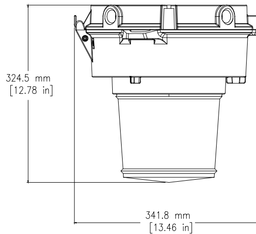
Side View - Refractor (LPGR5)
