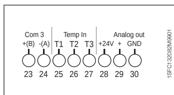
Figure 2: Terminal connection
