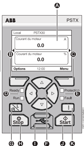
Figure 3 : Interface homme-machine
